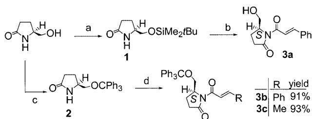
Scheme 2. Preparation of the imides 3a–c . a. t BuMe 2 SiCl, imidazole, DMAP, 97%; b. i. n BuLi, THF, ( E )-PhCHCHCOCl, -78 °C; ii. TBAF, THF, 94%; c. Ph 3 CCl, Et 3 N, DMAP, CH 2 Cl 2 , 73%; d. i. n BuLi, THF, -78 °C. ii. ( E )-PhCH=CHCOCl or ( E )-CH 3 CH=CHCOCl
