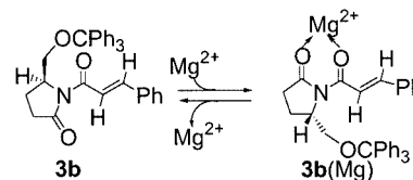
Scheme 1. Chelation of a magnesium ion to the imide 3b
