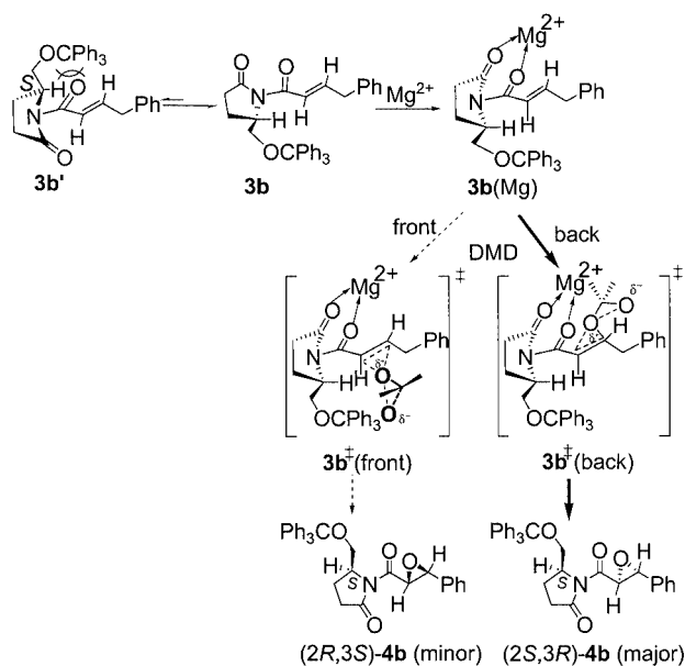
Scheme 5. Proposed mechanism for the diastereoselective DMD epoxidation of imide 3b through chelation of a magnesium ion to the carbonyl/carbonyl functionalities
