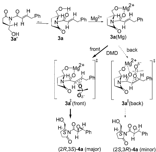
Scheme 4. Proposed mechanism for the diastereoselective DMD epoxidation of imide 3a through chelation of a magnesium ion with the hydroxy/carbonyl functionalities
